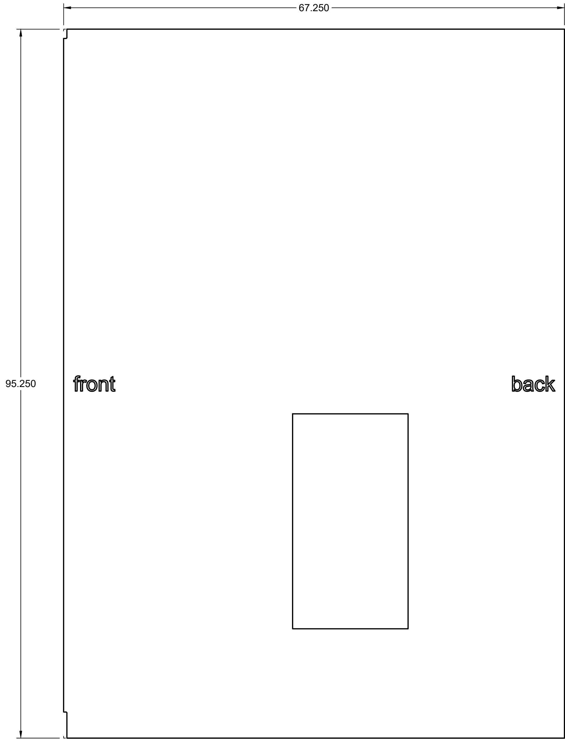
SIDE VIEW
